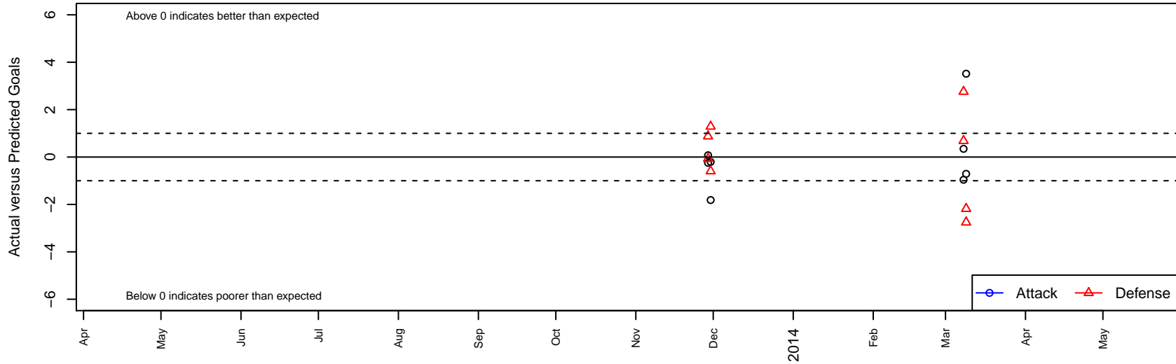
Impact United B00 Dots are actual minus expected GF (blue circles) and GA (red triangles). Blue line is smoothed change in attack strength. Red is smoothed change in defense strength.
